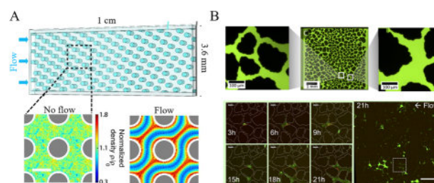
Fig. 17 Microfluidic devices featuring porous media geometries. (A) Comparison of the distribution of bacterial trajectories without flow and with flow condition in a homogenous microfluidic porous media chip, 308 colored lines indicate density patterns, black arrows indicate mean flow directions (reproduced with permission from the author). (B) Fluorescent images of Pantoaea cells growing in the heterogeneous porous network. To mimic realistic surroundings, the network not only has constriction points smaller than a bacterium's cell size but also larger, highly connected pore spaces 309 (reproduced with permission under a CC-BY Creative Commons license, Copyright 2019, Public Library of Science).
